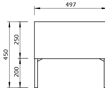
METALIC LEGS
