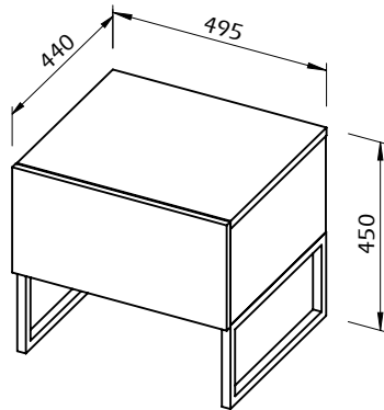
METALIC LEGS
