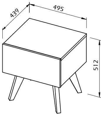
WOODEN LEGS
